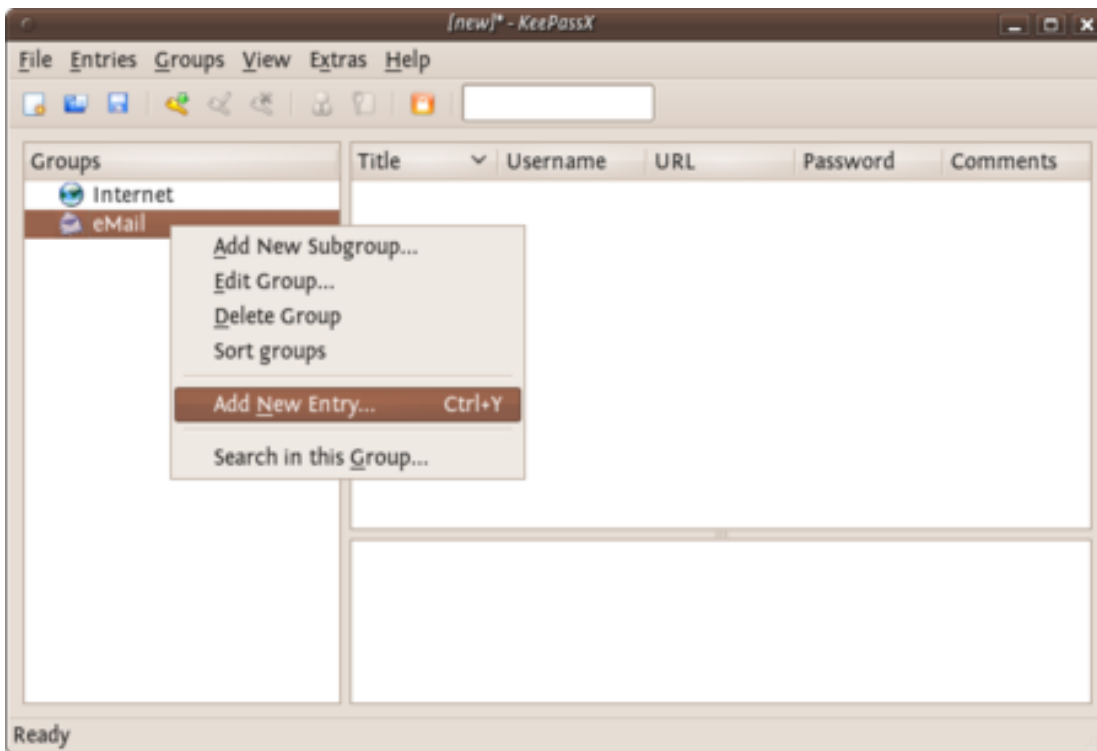
Figure 9.19: Password Manager
