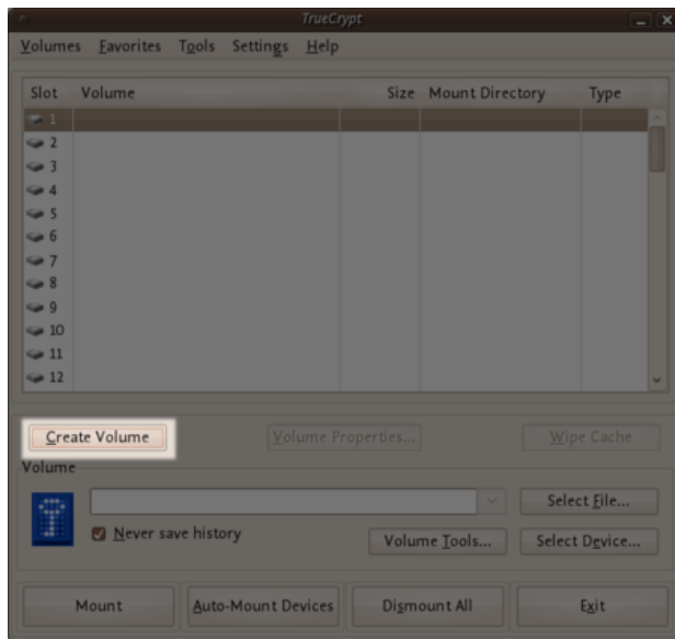
Figure 11.30: Hidden volumes
