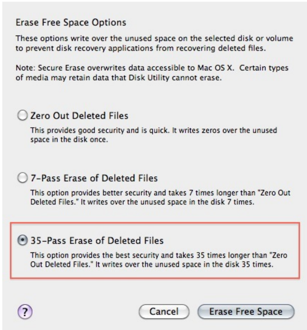
Figure 11.41: Destroying data
