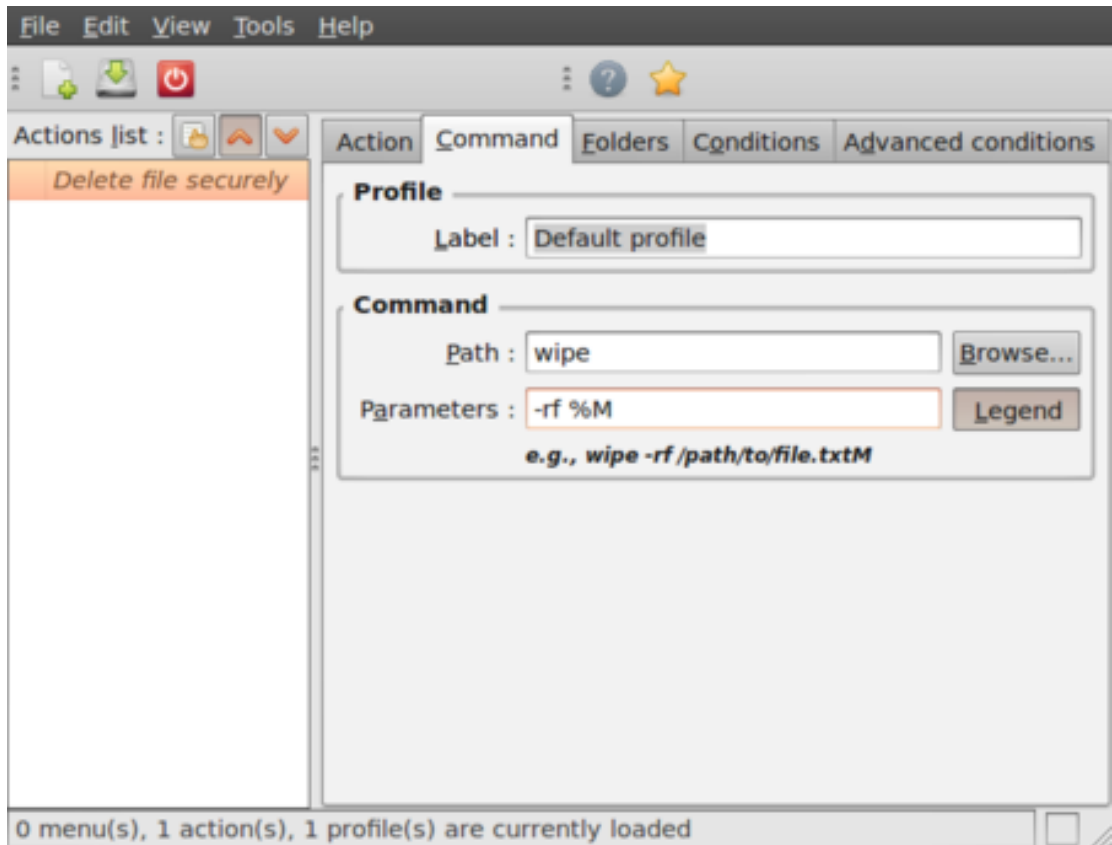
Figure 11.47: Destroying data
