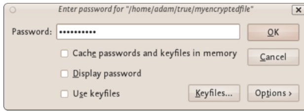
Figure 11.27: Using TrueCrypt
