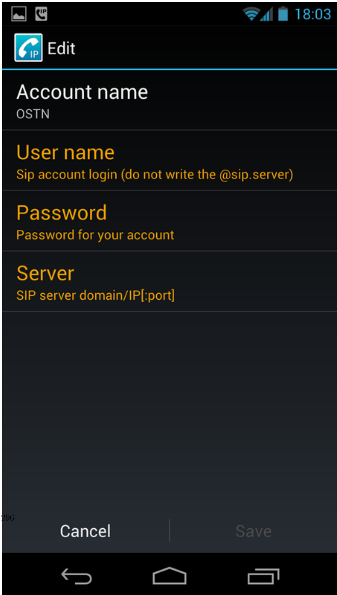
Figure 12.2: OSTN
