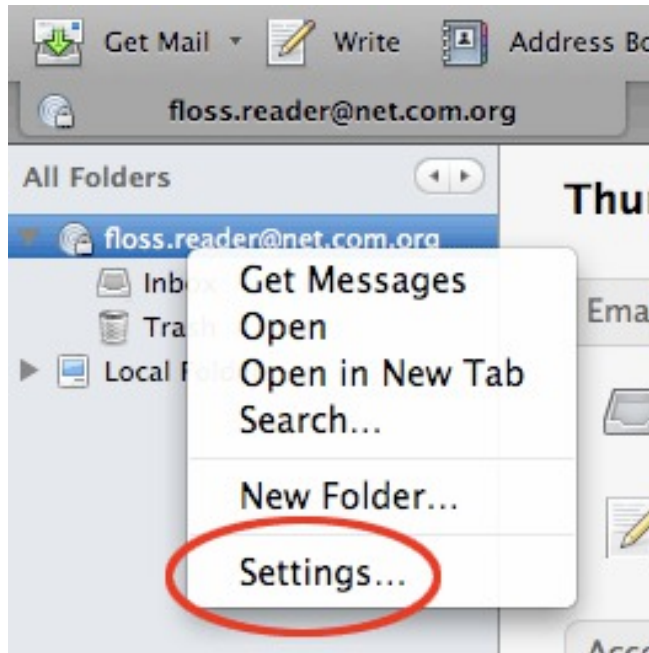
Figure 6.26: Thunderbird Security
