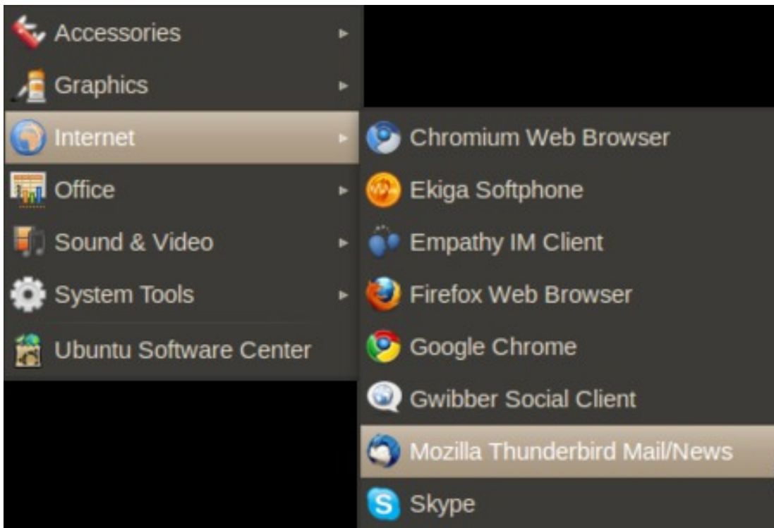
Figure 6.8: Thunderbird Install
