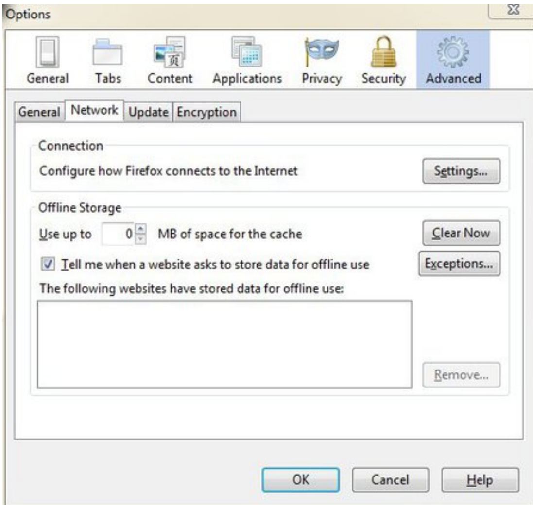
Figure 14.2: I2P
