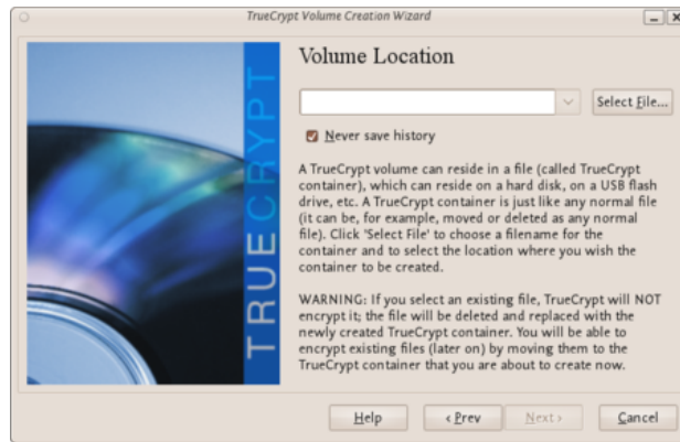
Figure 11.32: Hidden volumes
