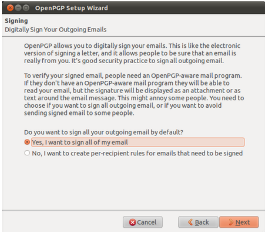
Figure 7.21: GPG Keys
