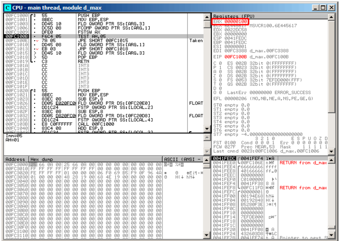
Figure 1.75: OllyDbg: FNSTSW executed
