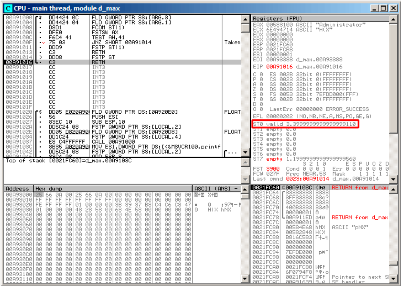
Figure 1.82: OlllyDbg: FSTP is executed
