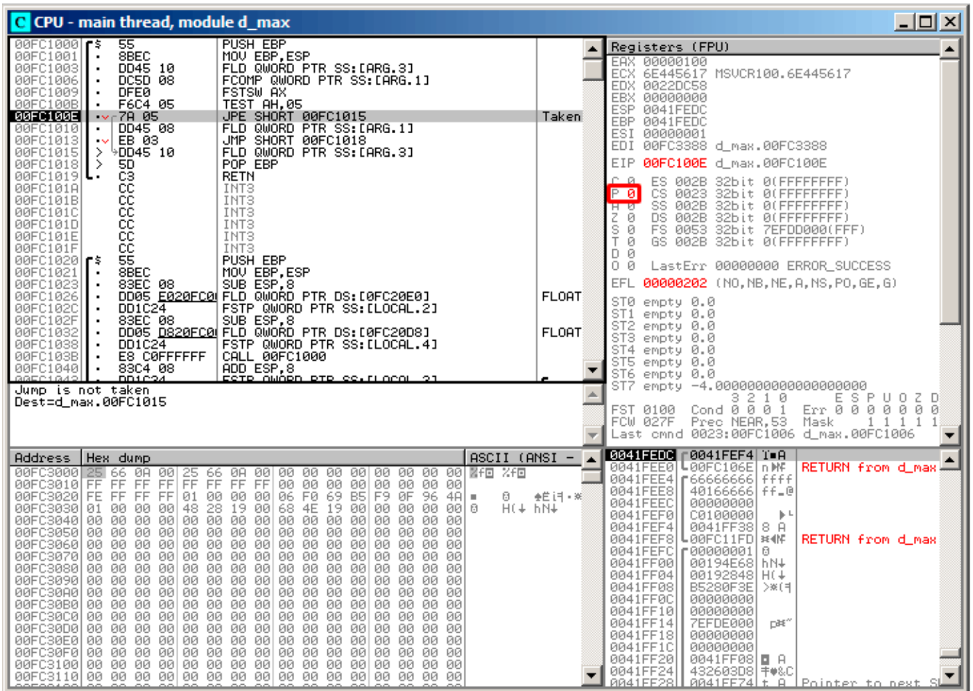
Figure 1.76: OllyDbg: TEST executed
