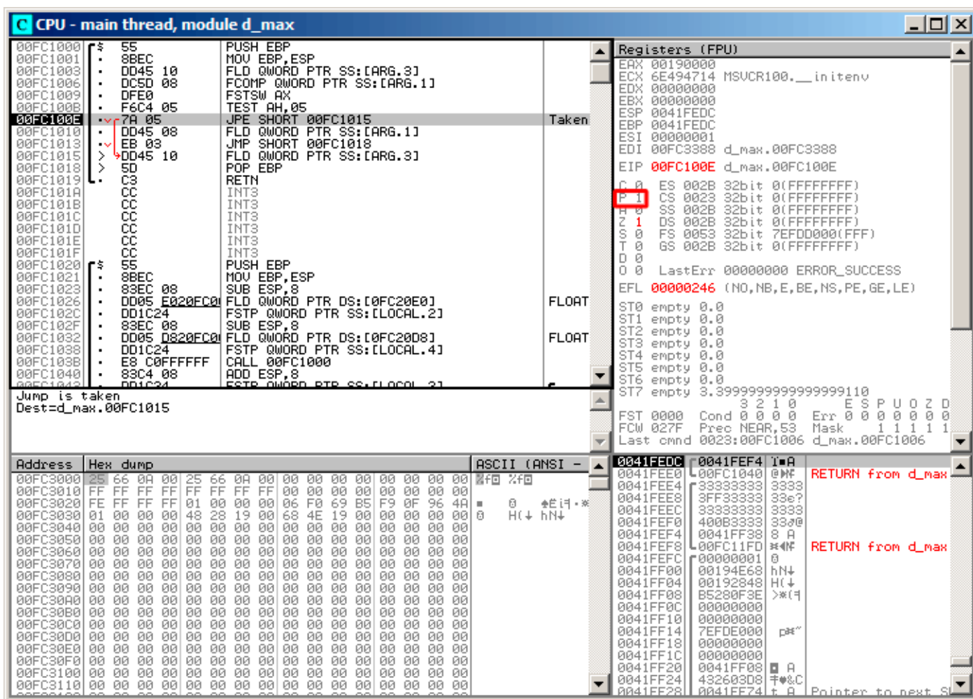
Figure 1.71: OllyDbg: TEST has been executed
